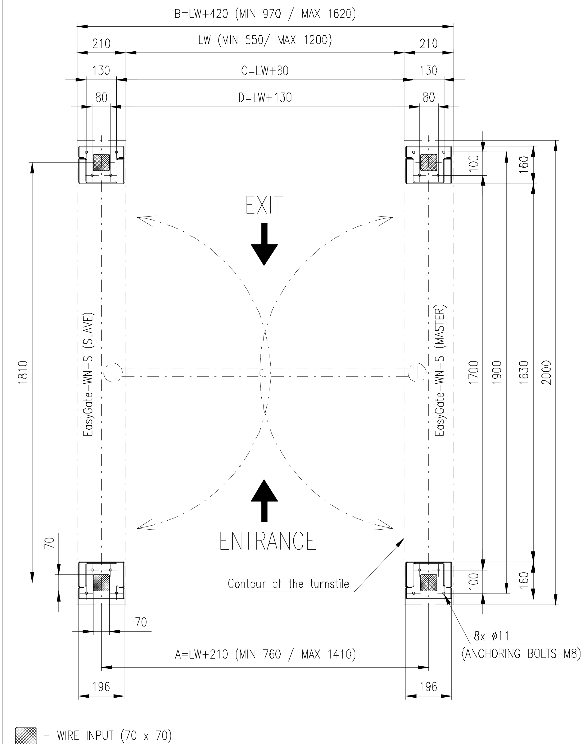
Anchoring dimensions
